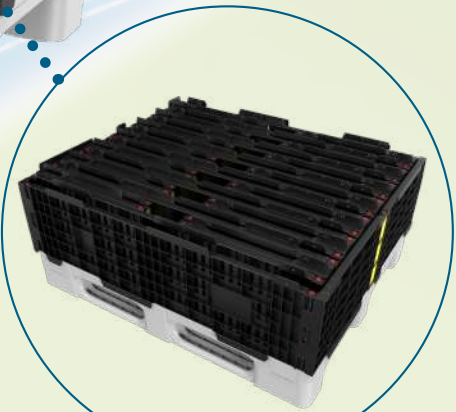
Big image: 9728001 Pallet collar on top of a BaYoPal® pallet Small image: folded pallet collars in an unfolded unit to save space during return trips
